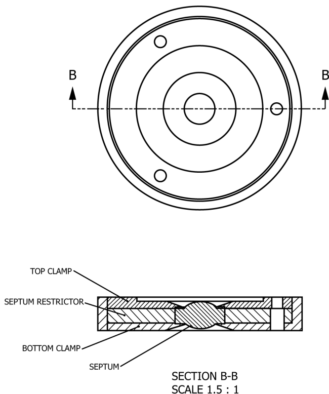
FIG. 4 Cross-Section of Clamping Device with Septum
