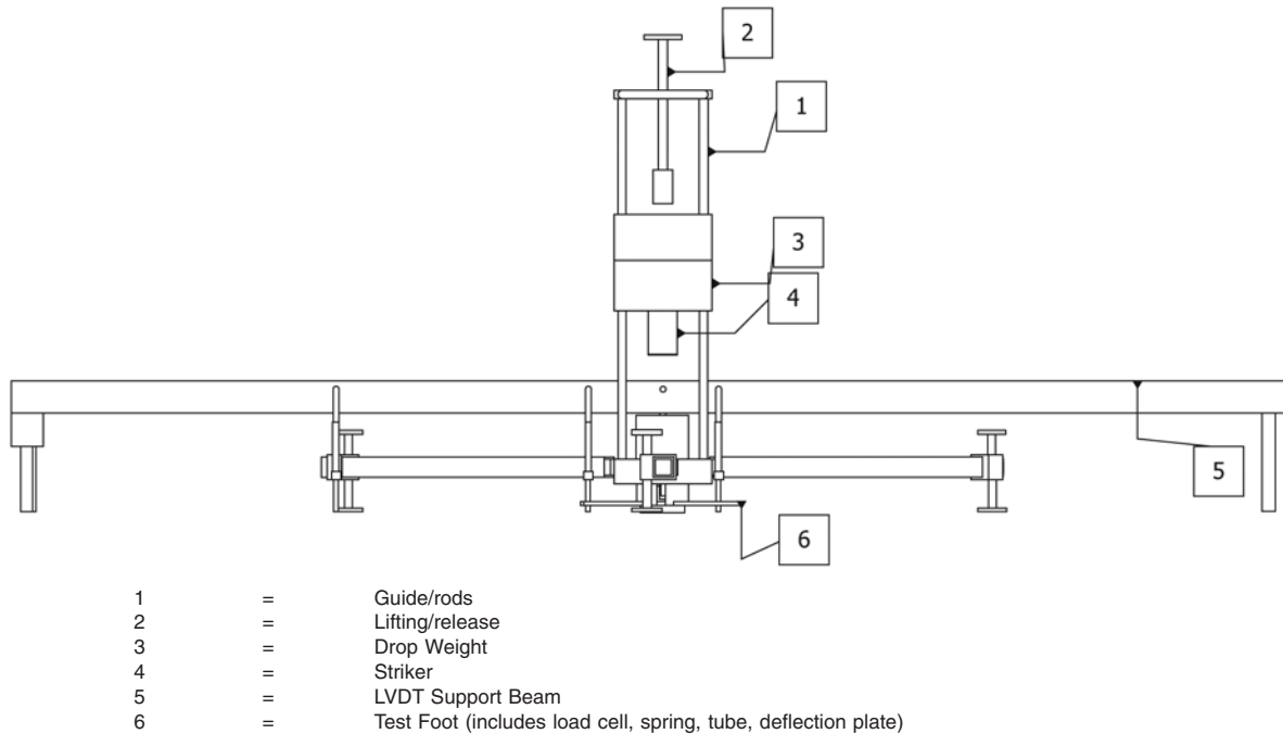
FIG. 1 Vertical Deformation Test Apparatus – Front View
