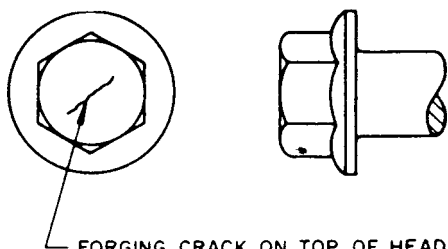
FIG. 2 Typical Forging Cracks
