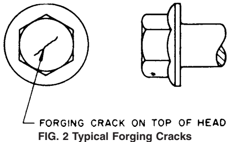
FIG. 2 Typical Forging Cracks
