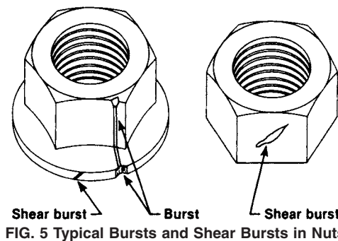
FIG. 5 Typical Bursts and Shear Bursts in Nuts
