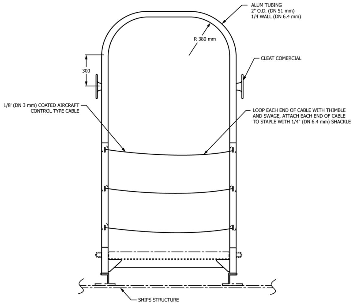
FIG. 2 Front View
