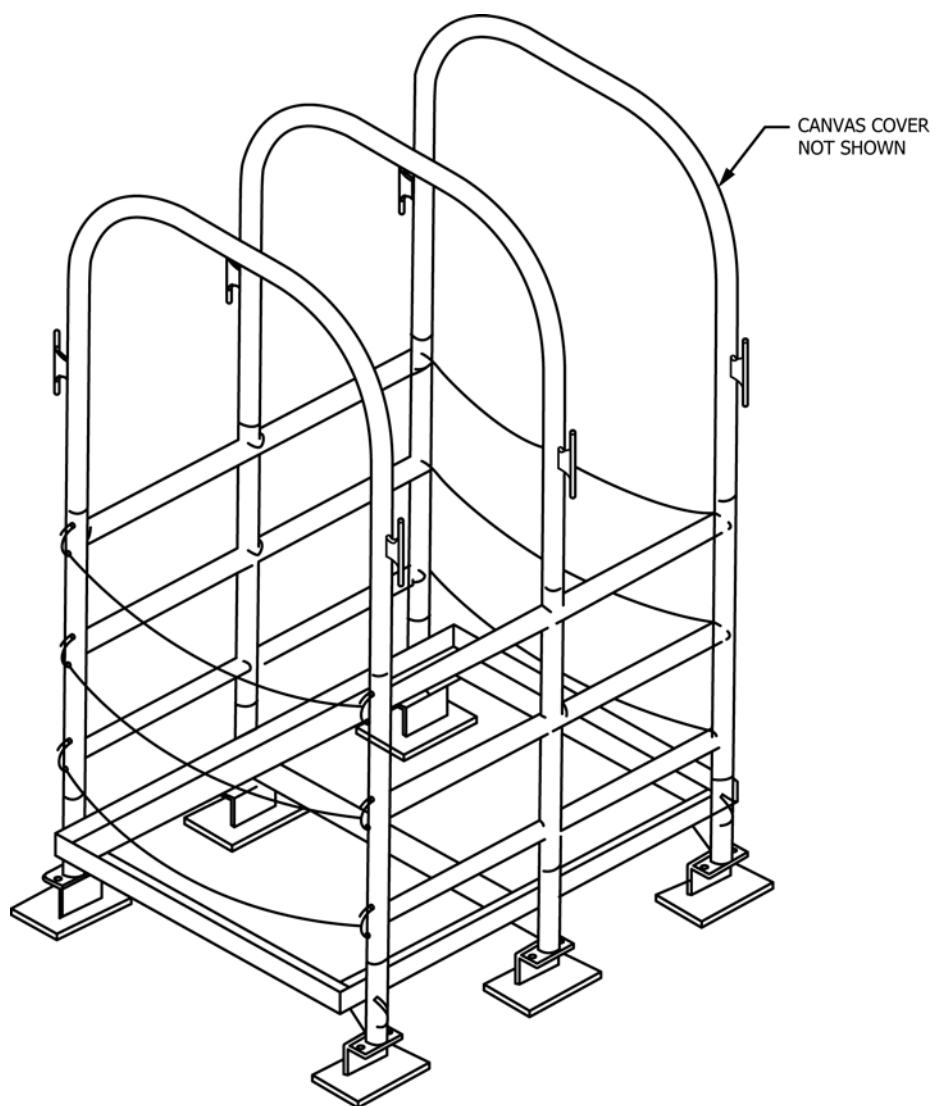
FIG. 1 Pilot Platform
