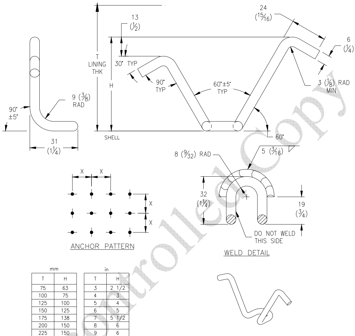
Figure 1 Double Hook Vee Anchor
