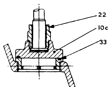
Flat seat type disk showing soft seal ring in disk or in seat ring
