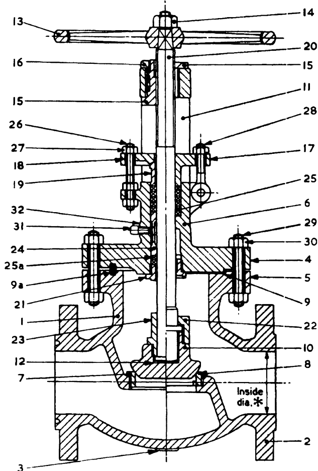
Typical half-sections showing alternative designs, including ball type disk
