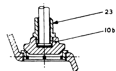
Narrow seat type disk
