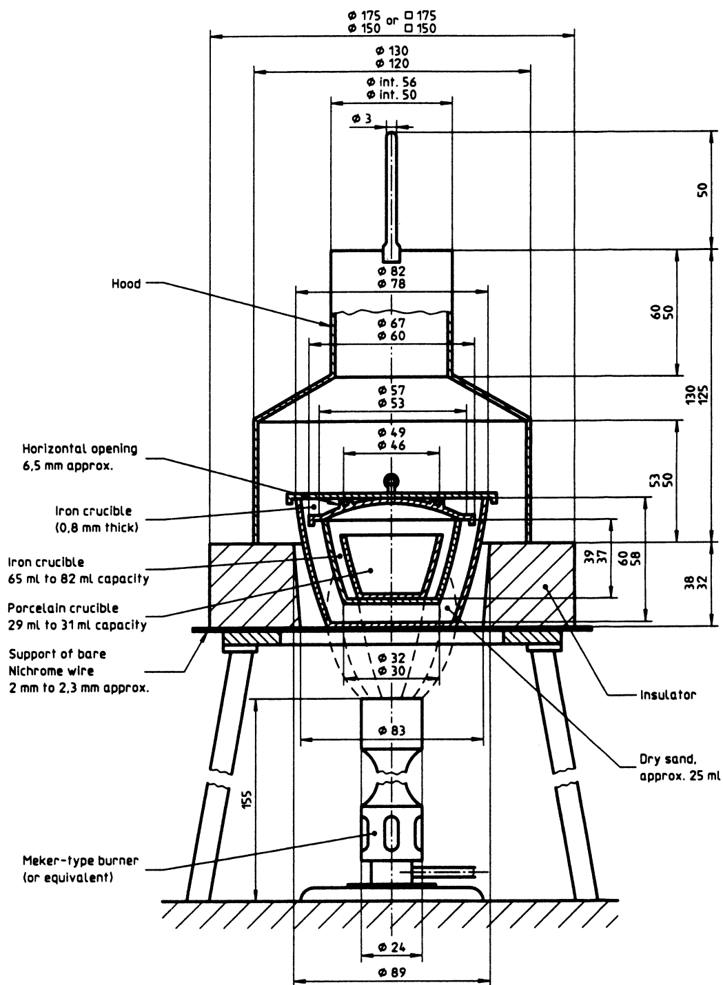
Figure 1 — Apparatus for determining Conradson carbon residue
