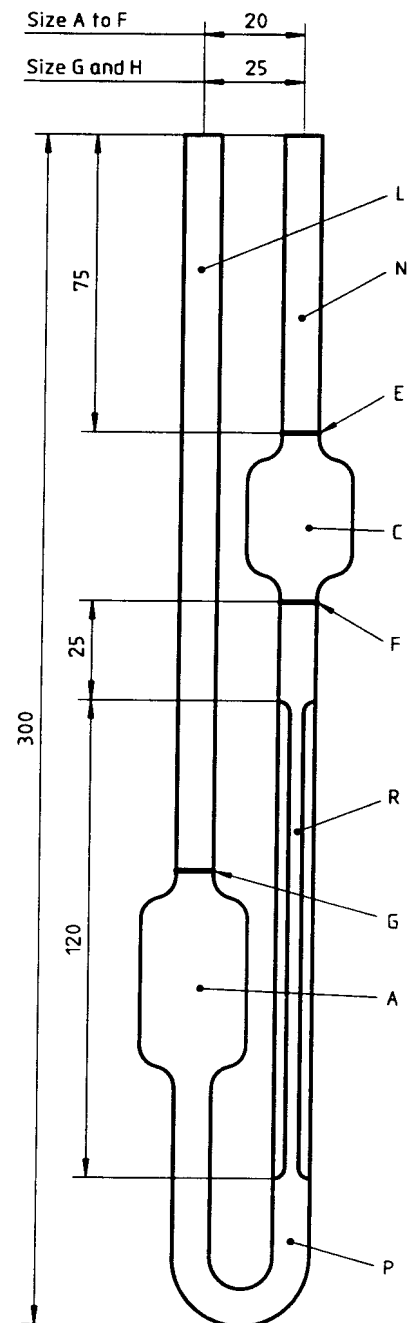
Figure A.3 — BS/U-tube viscometer
