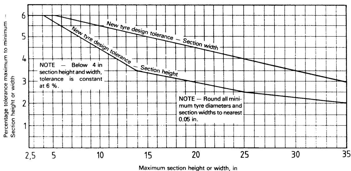
Figure 4 — New aircraft tyre section height and width — Dimensional tolerances (inches) 2)
