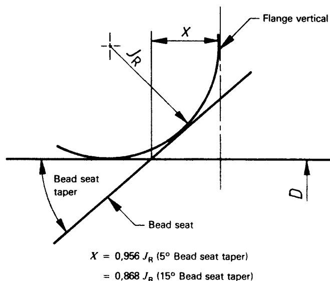
Figure 8 — Dimensioning of D specified rim diameter
