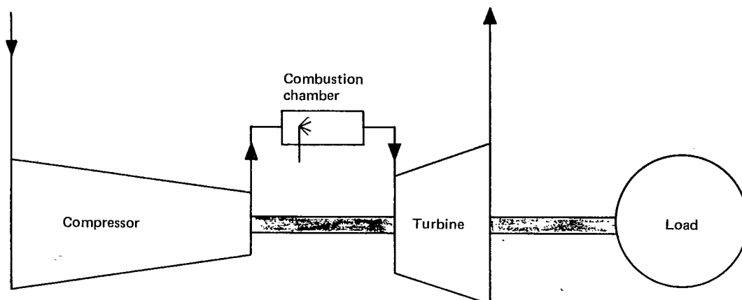
a) Simple cycle, single-shaft gas turbine
