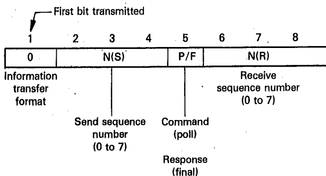
Figure 4 — Information transfer format of control field bits
