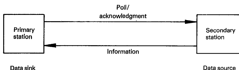
Figure 2 — Unbalanced data link configuration (case 2)
