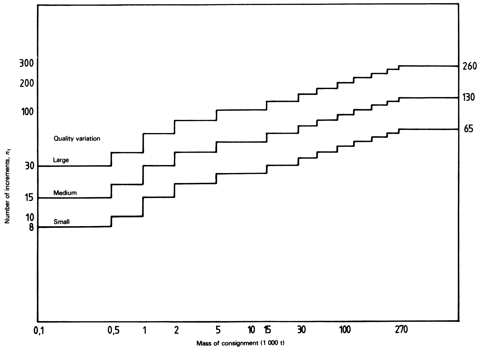
Figure 2 — Minimum number of increments required
