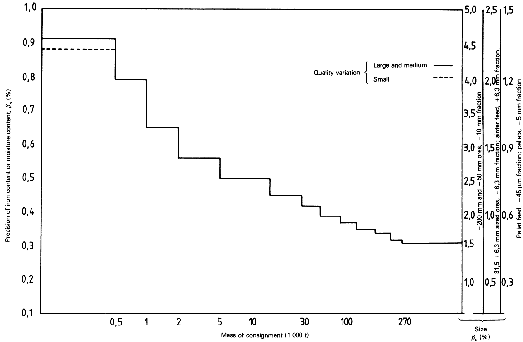
Figure 1 — The precision of sampling for each mass of consignment
