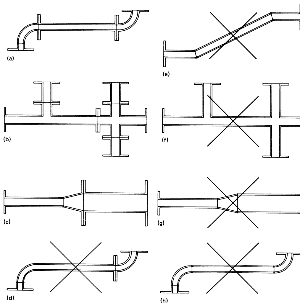
Figure 1. Pipework details
