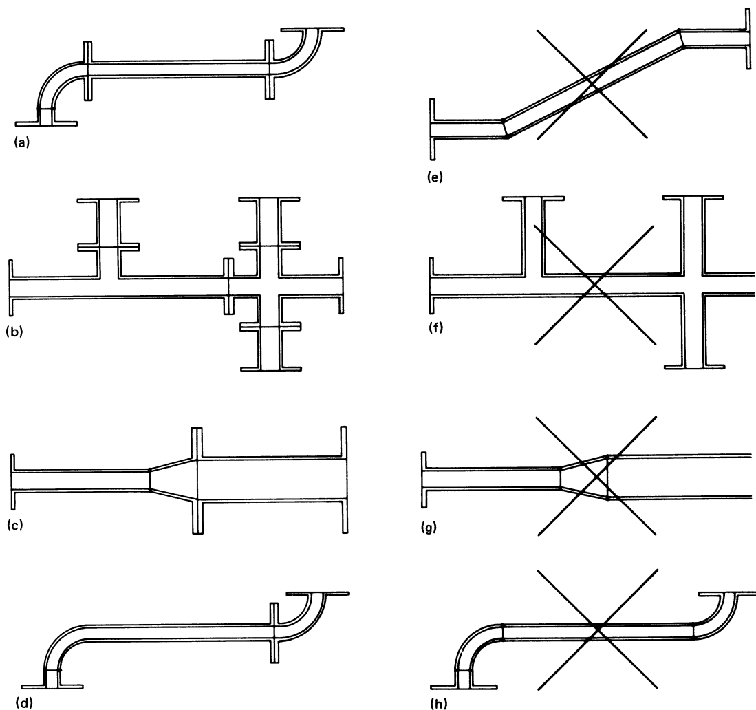
Figure 1 — Pipework details
