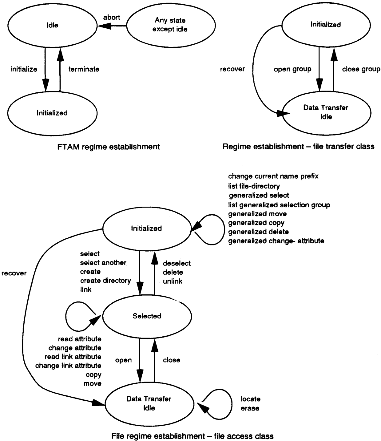
Figure 3 – Simplified State Diagram for successful activity (see Annex E)
