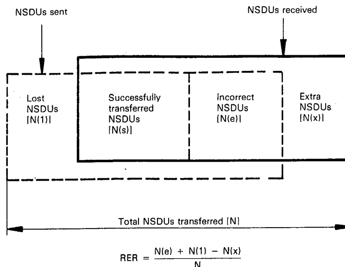
Figure 3 — Components of residual error rate
