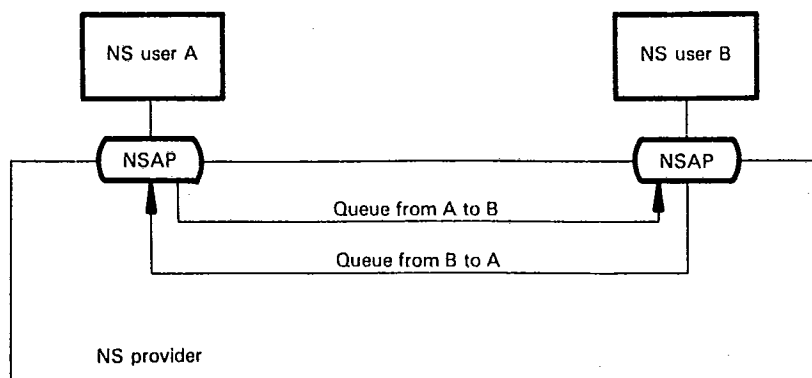
Figure 2 — Queue model of a Network Connection
