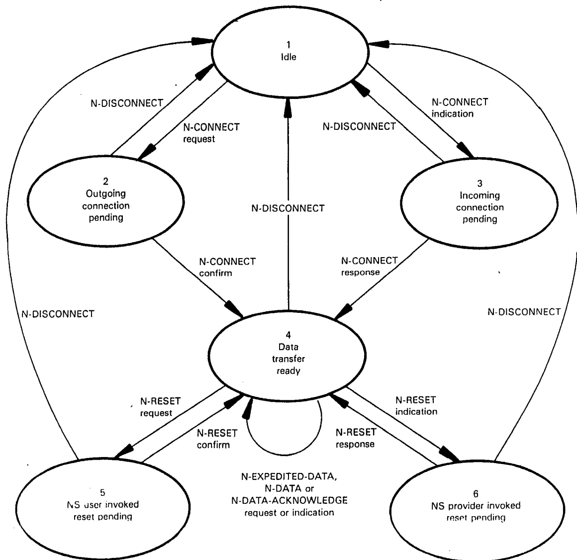
Figure 5 — State transition diagram for sequences of primitives at an NC endpoint
