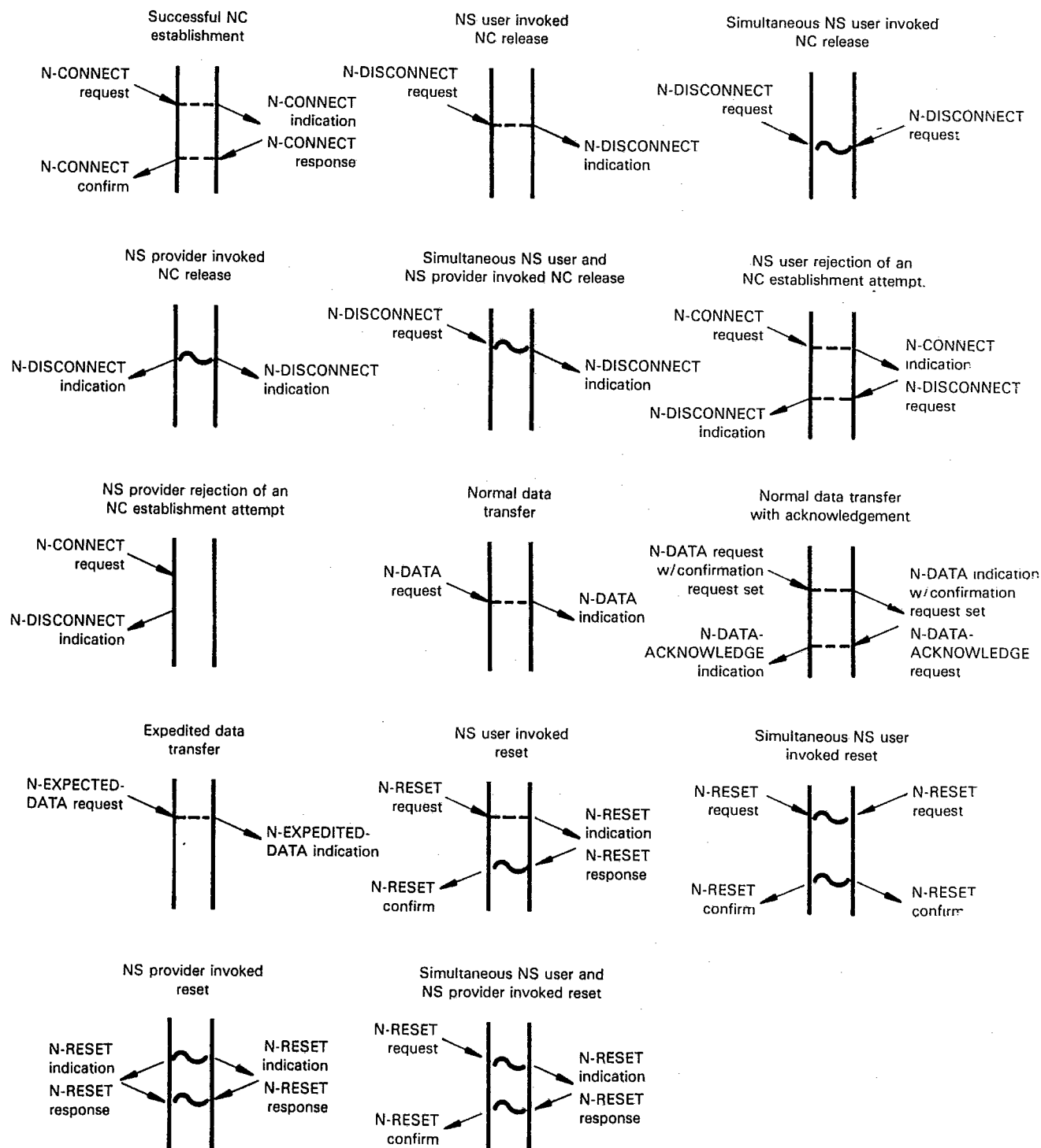
Figure 4 — Summary of Network Service primitive time sequence diagrams
