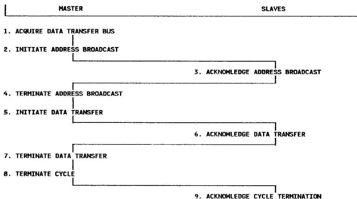
Fig. 2-7. - General flow of a SINGLE-TRANSFER cycle.
