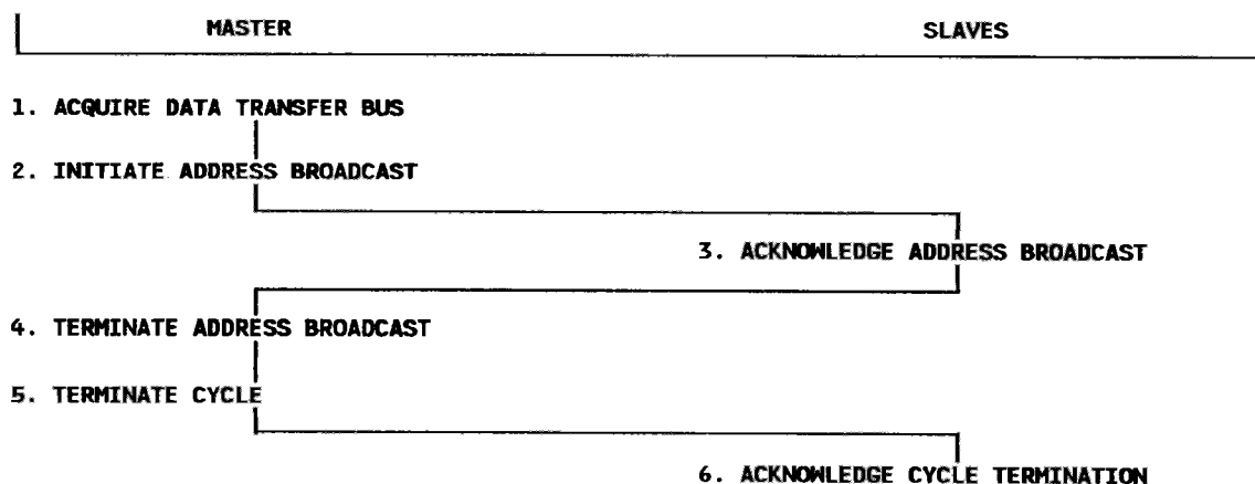
Fig. 2-5. - General flow of an ADDRESS-ONLY cycle.
