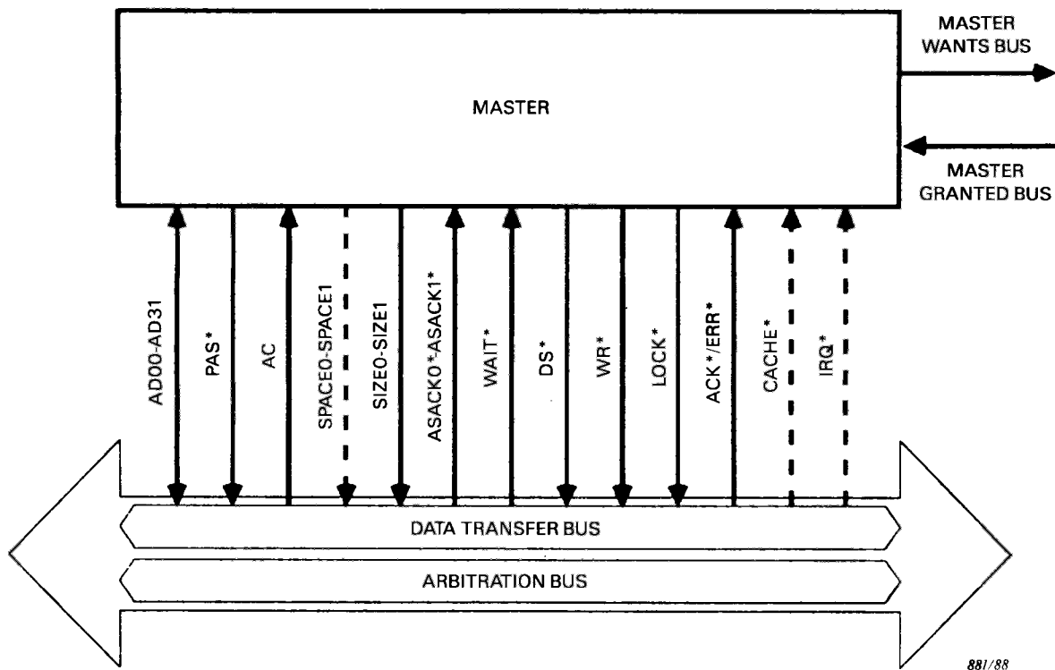
Fig. 2-2. - Block diagram: MASTER.
