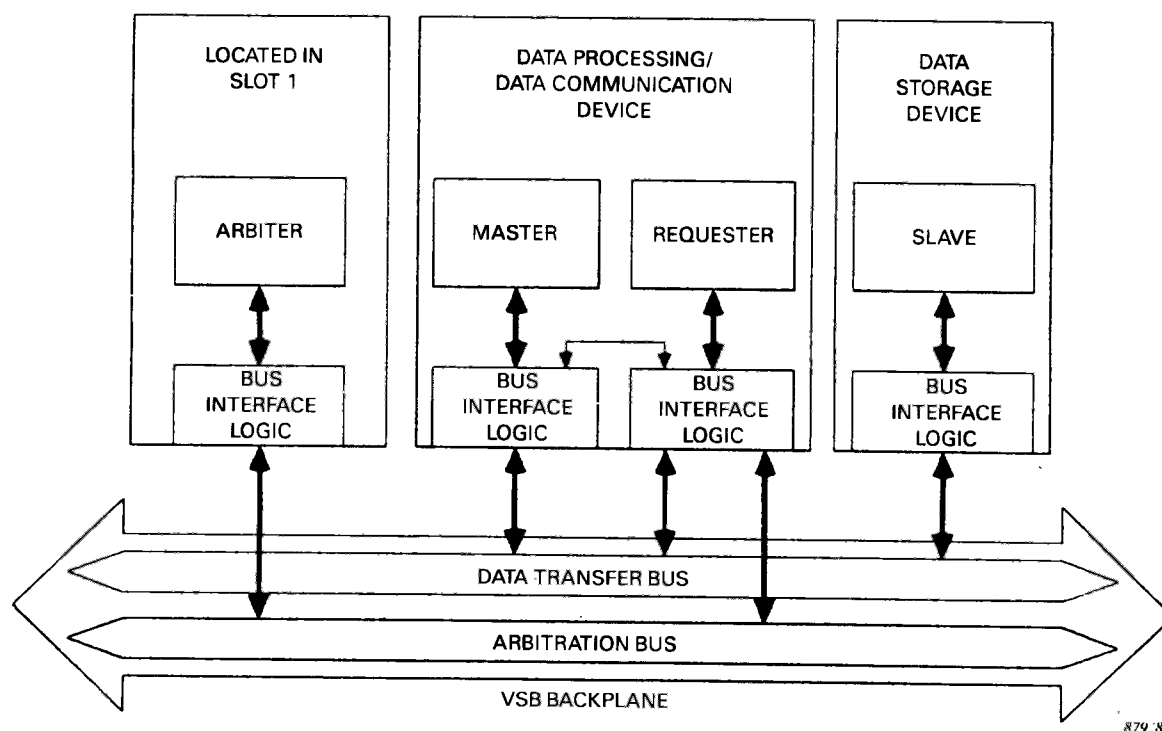
Fig. 1-1. - Functional modules and sub-buses defined by the VSB standard.
