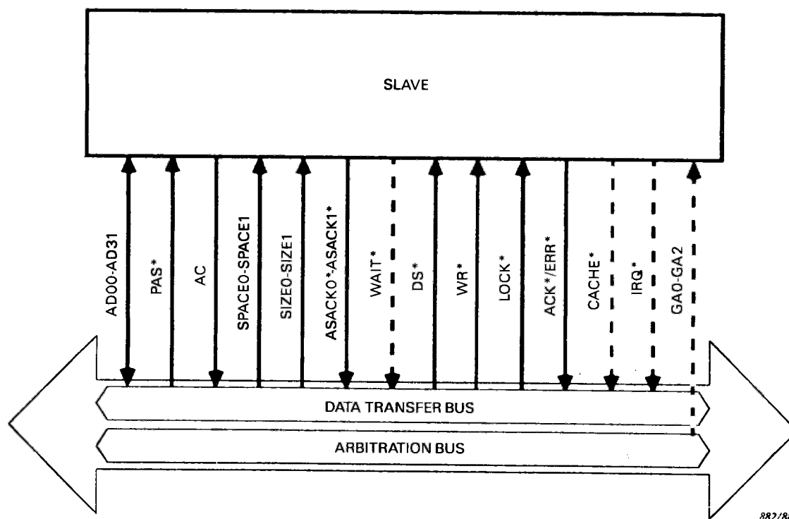
Fig. 2-3. - Block diagram: SLAVE.
