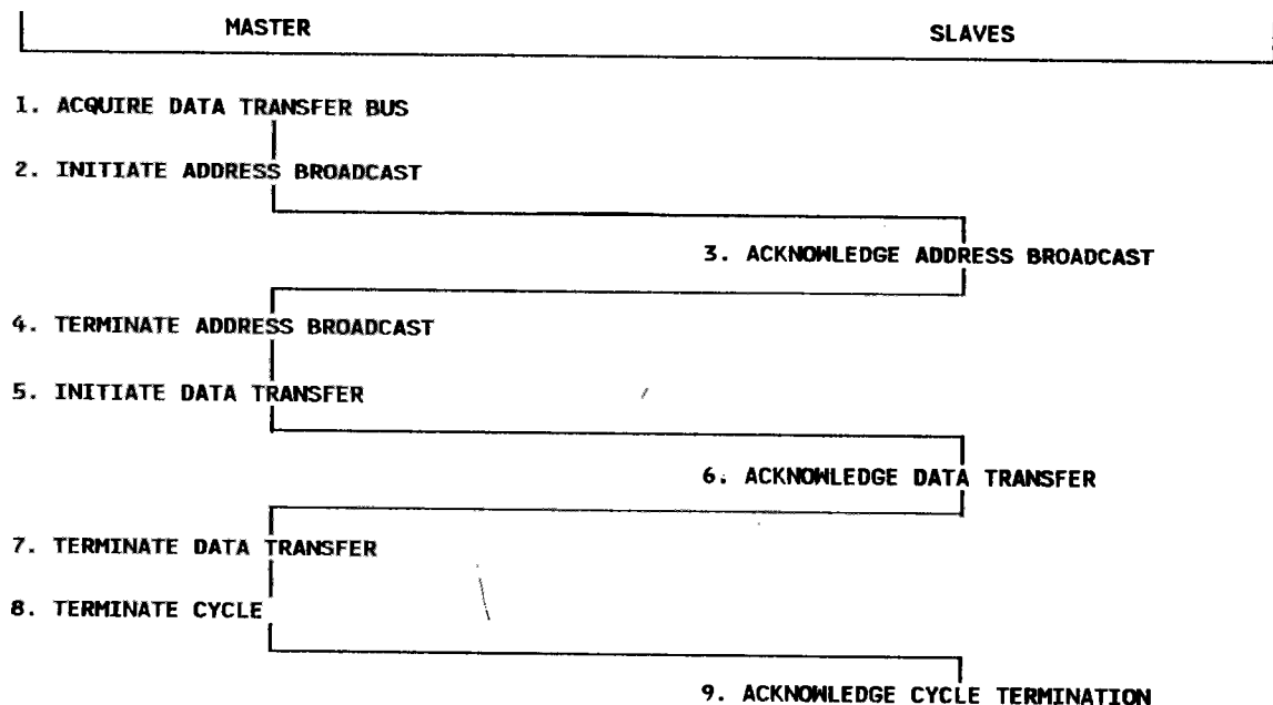
Fig. 2-4. - General flow of a VSB cycle.
