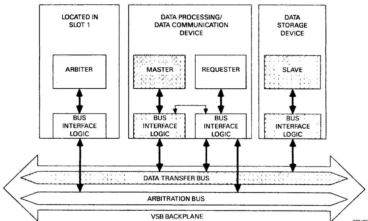
Fig. 2-1. - Data Transfer Bus functional block diagram.
