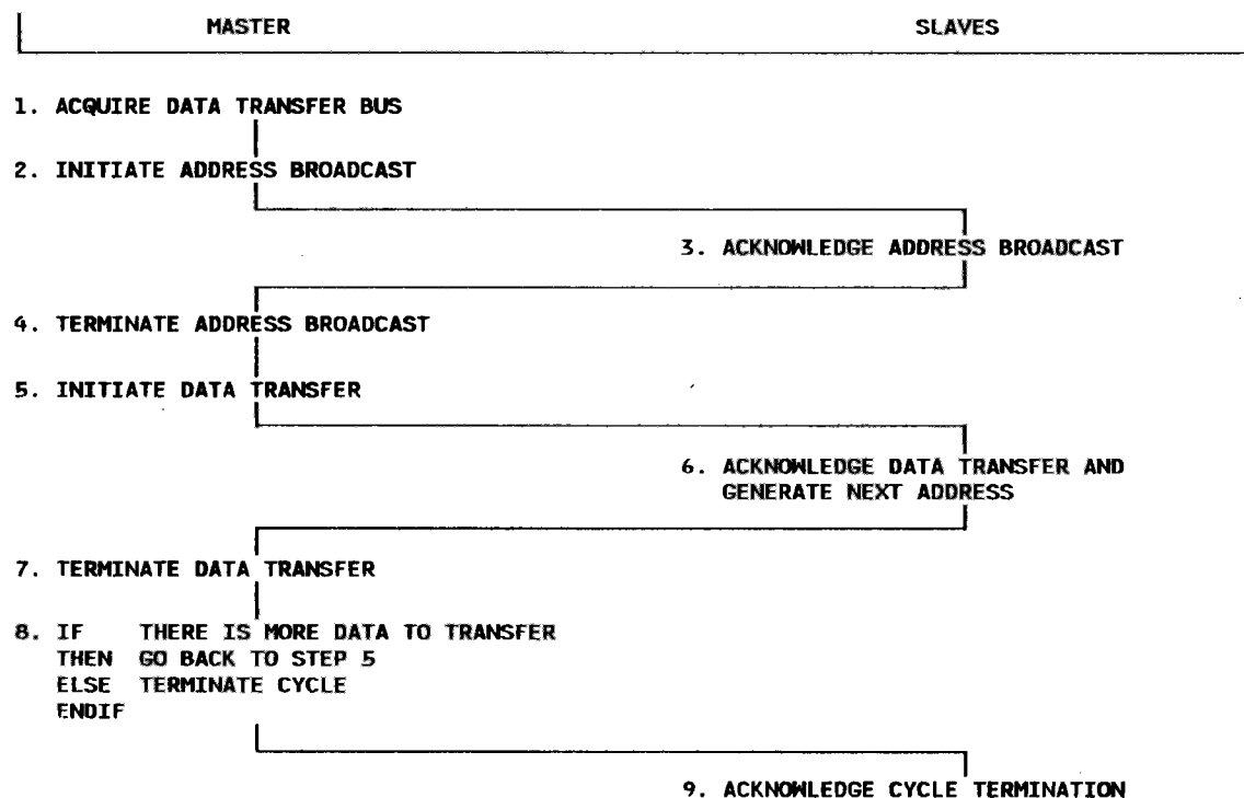
Fig. 2-8. - General flow of a BLOCK-TRANSFER cycle.
