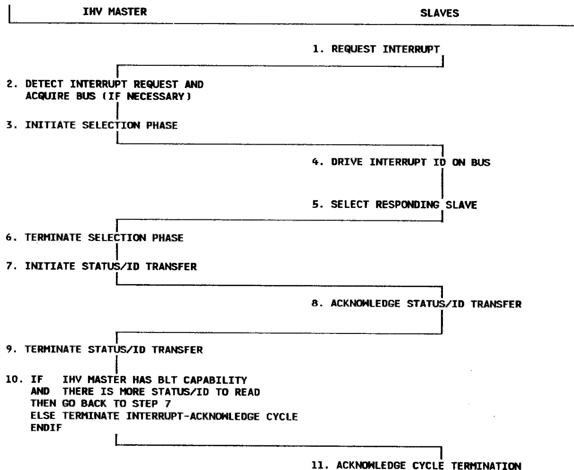
Fig. 2-9. - General flow of an INTERRUPT-ACKNOWLEDGE cycle.
