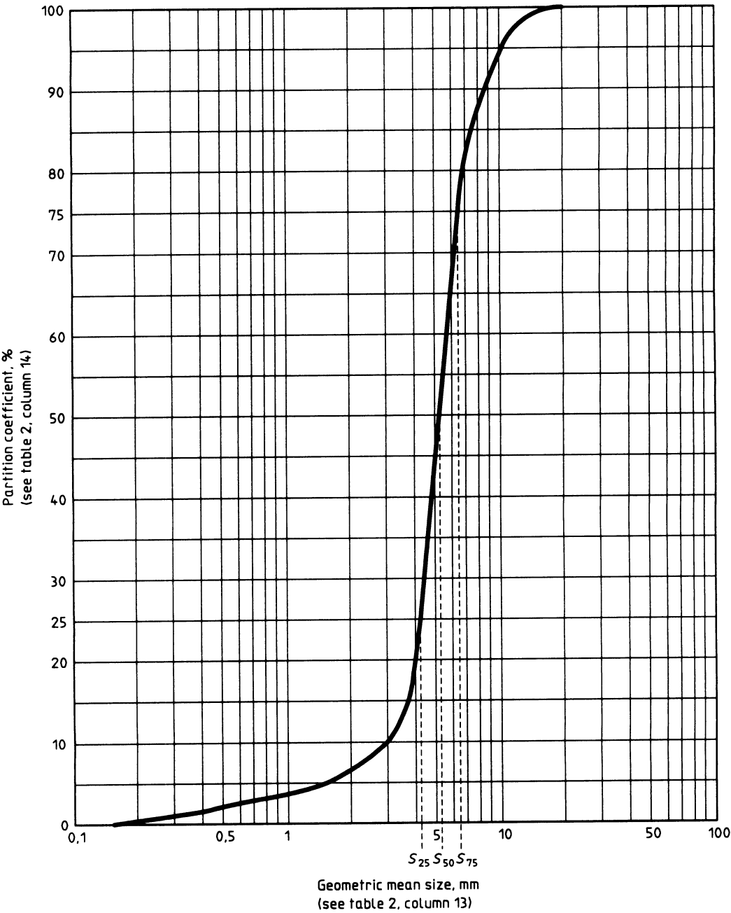
Figure 1 — Partition curve
