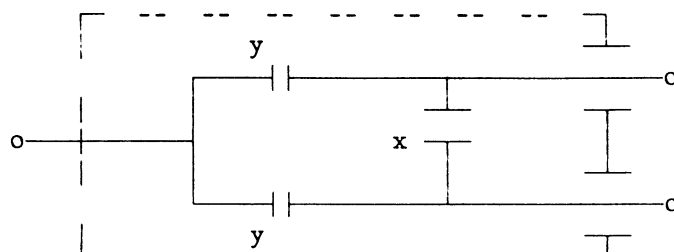
Figure 5b — Delta by-pass capacitor
