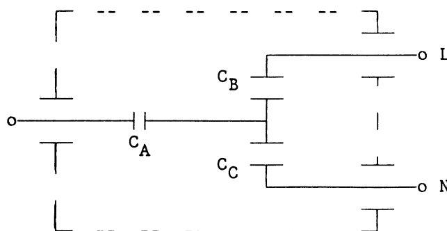
Figure 5c — Example of a T-connected by-pass capacitor
