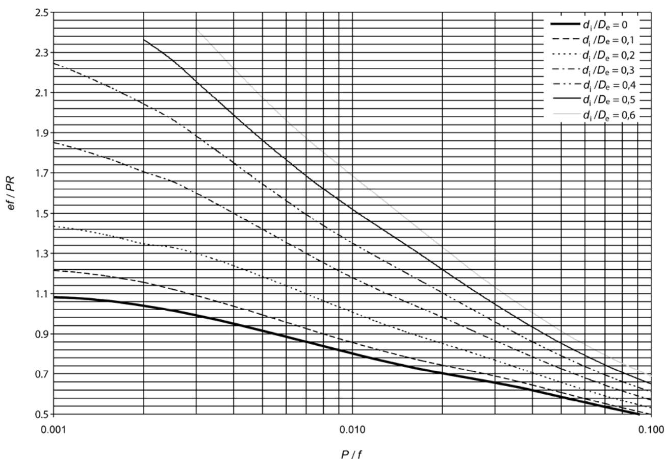
Figure 7.7-1 — Design ratio for Kloepper ends
