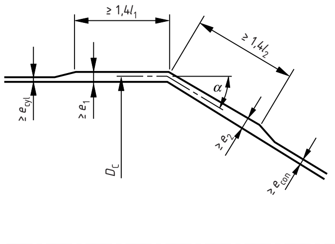
Figure 7.6-1 — Geometry of cone/cylinder intersection without knuckle — Large end
