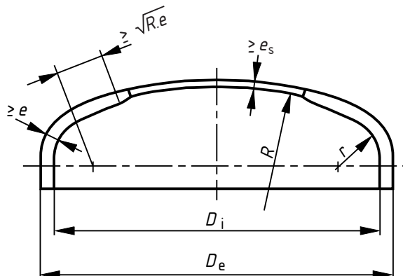
Figure 7.5-3 — Geometry of torispherical end
