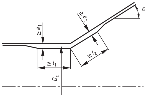
Figure 7.6-4 — Geometry of cone/cylinder intersection: small end
