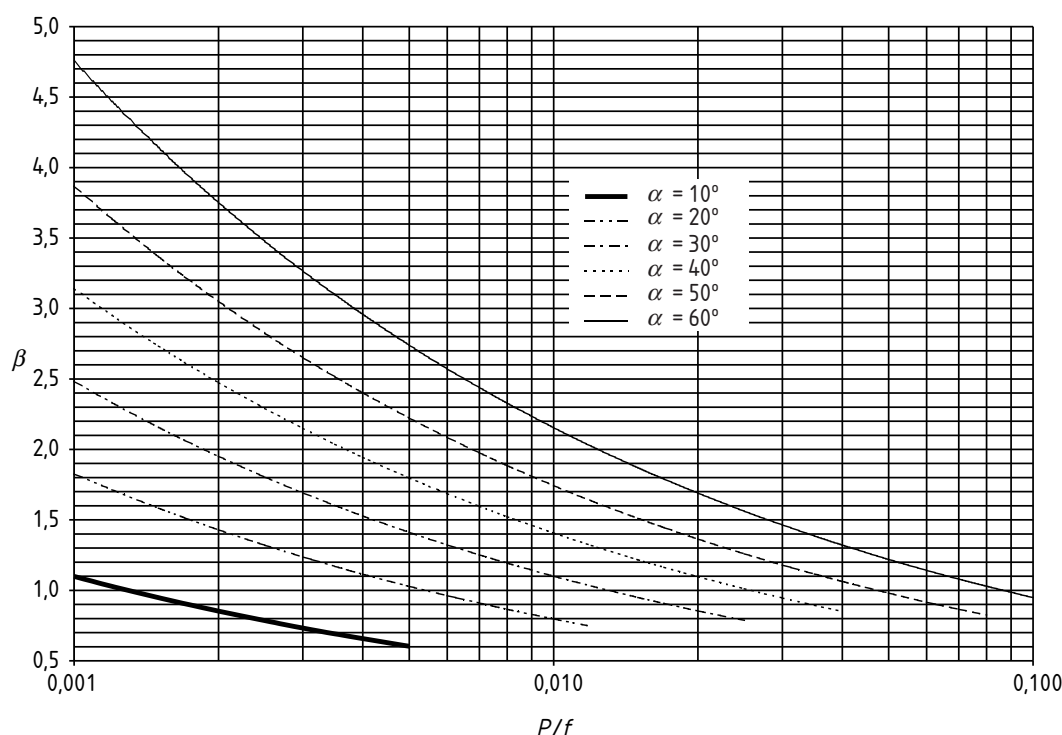
Figure 7.6-3 — Values of coefficient \beta for cone/cylinder intersection without knuckle
