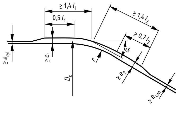
Figure 7.6-2 — Geometry of cone/cylinder intersection with knuckle — Large end
