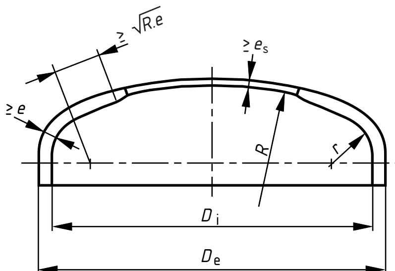
Figure 7.5-3 — Geometry of torispherical end
