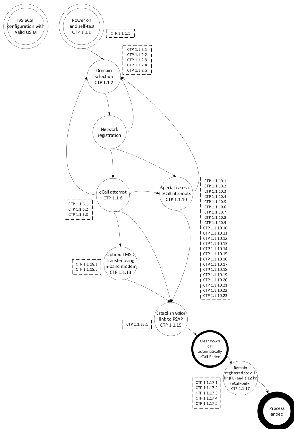
Figure 9 — State transitions for eCall IVS in hybrid circuit switched/packet switched network environments with associated CTP references
