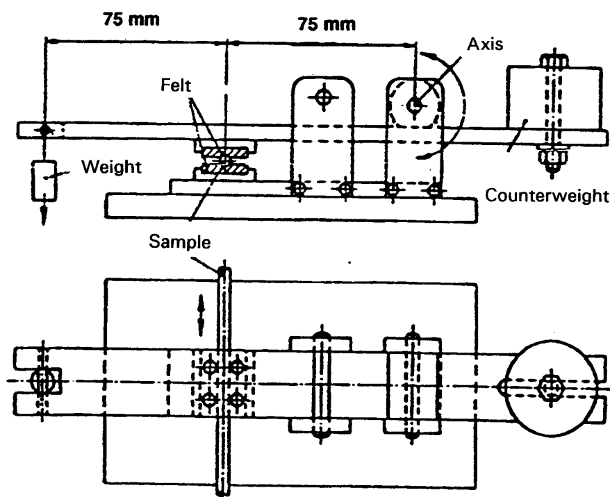
Figure 3 - Test set-up
