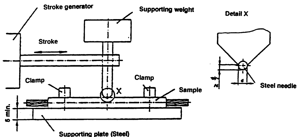
Figure 2 - Test set-up
