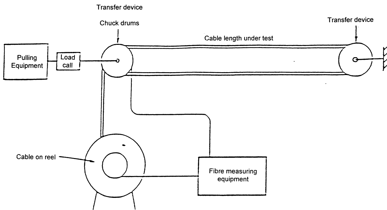
Fig. 101A - Tensile performance measuring apparatus with multiple pass of the cable on the ring
