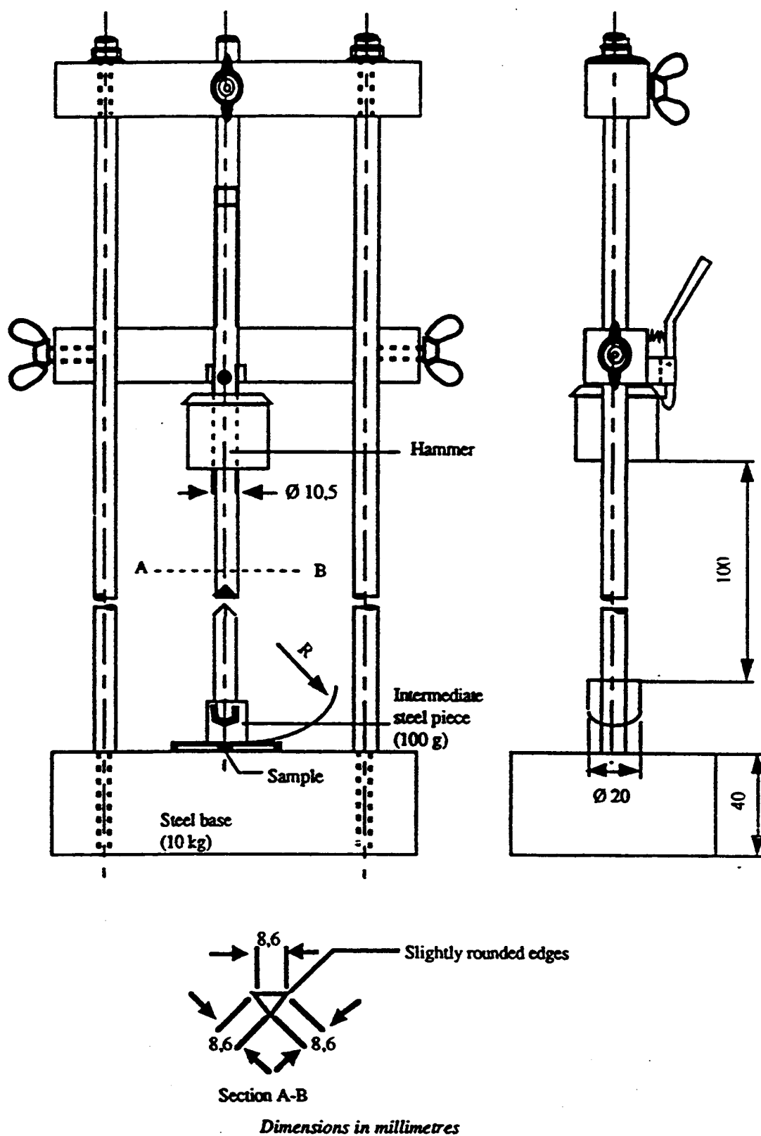
Figure 5 - Impact test
