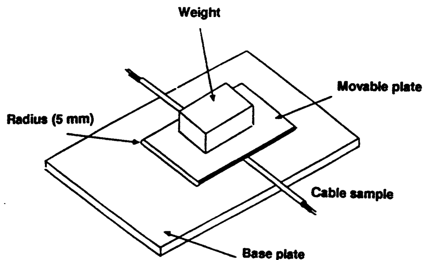
Figure 4 - Crush test
