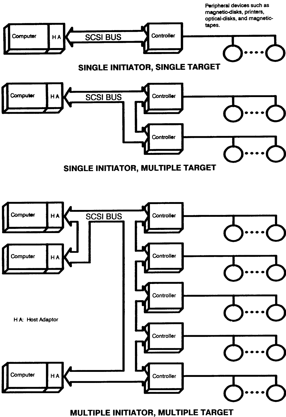
Figure 7 — Sample SCSI Configurations
