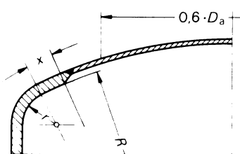
Figure 8 — Dished end with knuckle and crown of unequal wall thickness
