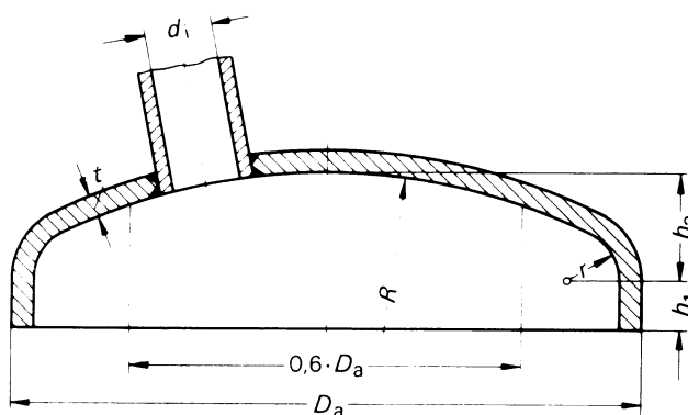
Figure 7 — Dished end with branch
