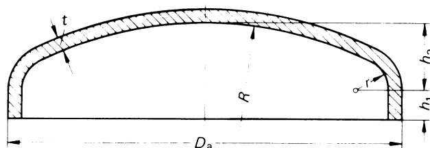
Figure 6 — Dished end
