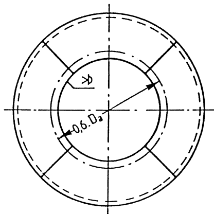
Figure 11 — Welded dished end from crown and knuckle components inside 0,6D_a : v = 1,0
