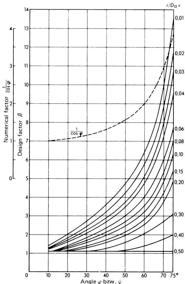
Figure 5 — Design factor \beta and numerical factor 1/\cos \varphi
