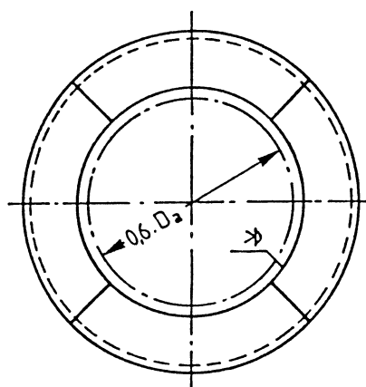
Figure 12 — Welded dished end from crown and knuckle components outside 0,6D_a : v = 0,75 resp. 1,0
