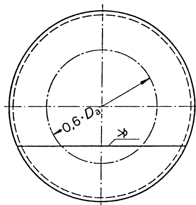
Figure 10 — Welded joint inside 0,6D_a : v = 1,0
