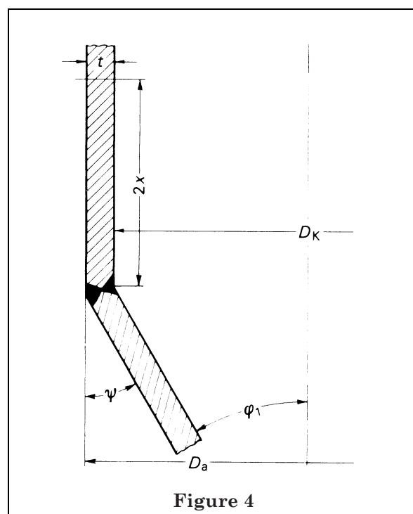
Figure 1 to Figure 4 — Typical connections between cylindrical and conical shells
