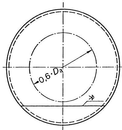
Figure 9 — Welded joint outside 0,6D_a : v = 0,75 resp. 1,0
