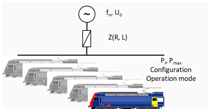
Figure 4 — Simplified combined system with scaling of number of traction units to fulfil least requirement on total installed maximum power at wheel.
