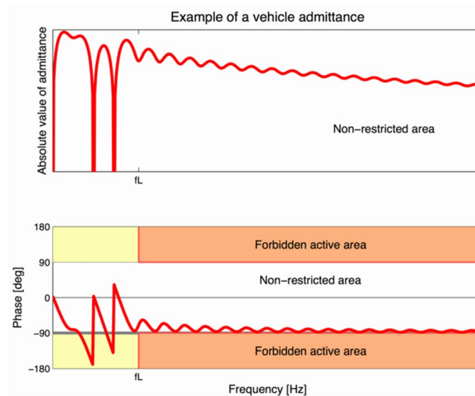
Figure 2 — Example of a frequency response of input admittance of a traction unit and forbidden zones of phase angle
