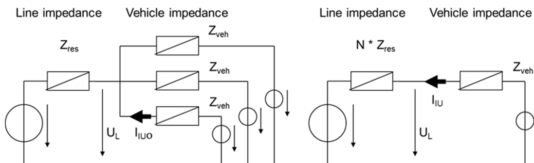
Figure 5 — Illustration of how the calculation of k_Z(f_0) is done
