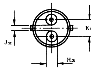
Circular contacts Contacts circulaires
