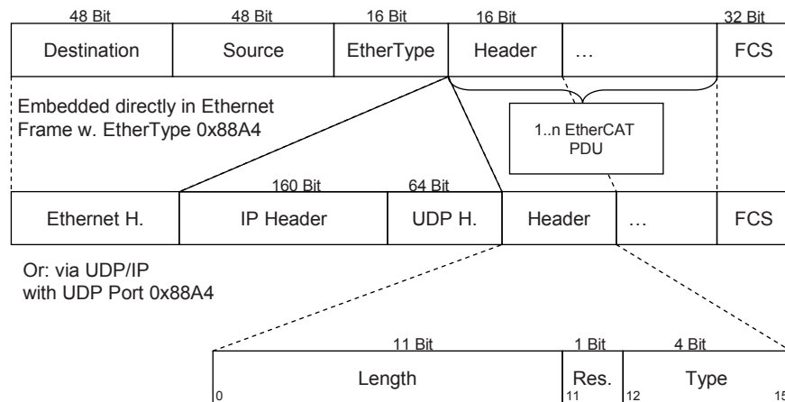
Figure 3 – Frame structure
