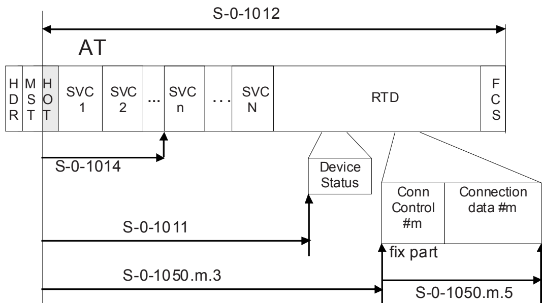
Figure 3 – Offsets within AT payload
