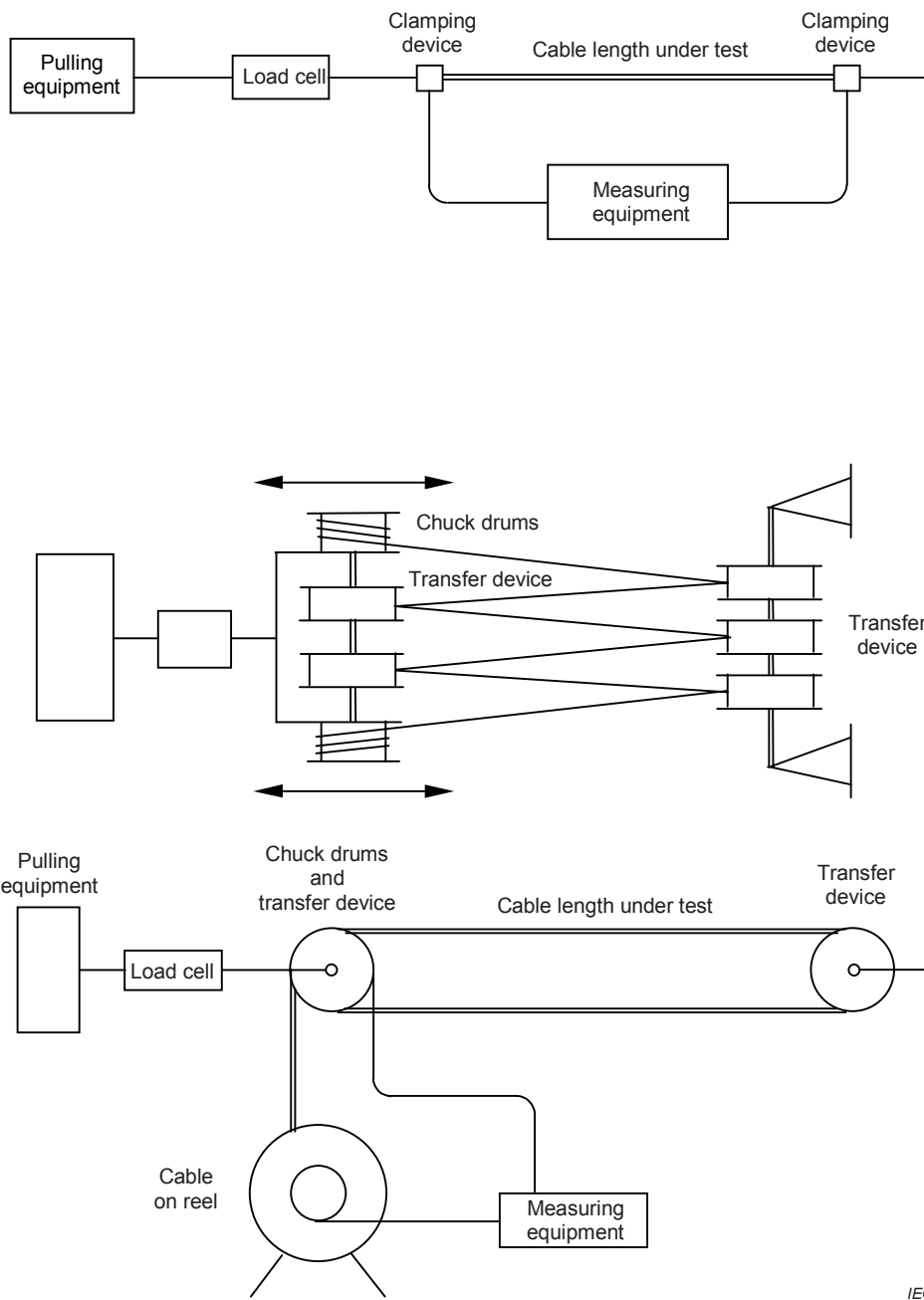
Figure 3 – Tensile performance measuring apparatus
