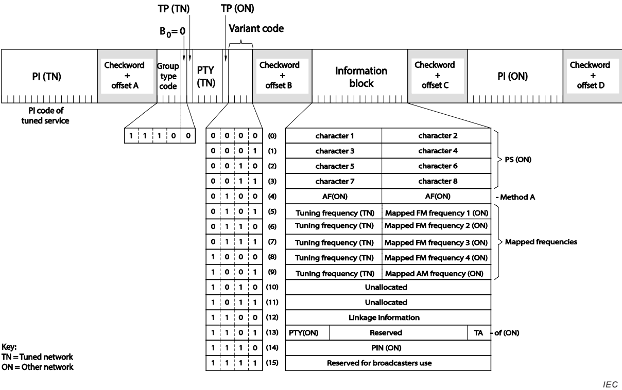
Figure 37 – Enhanced other networks information – Type 14A groups
