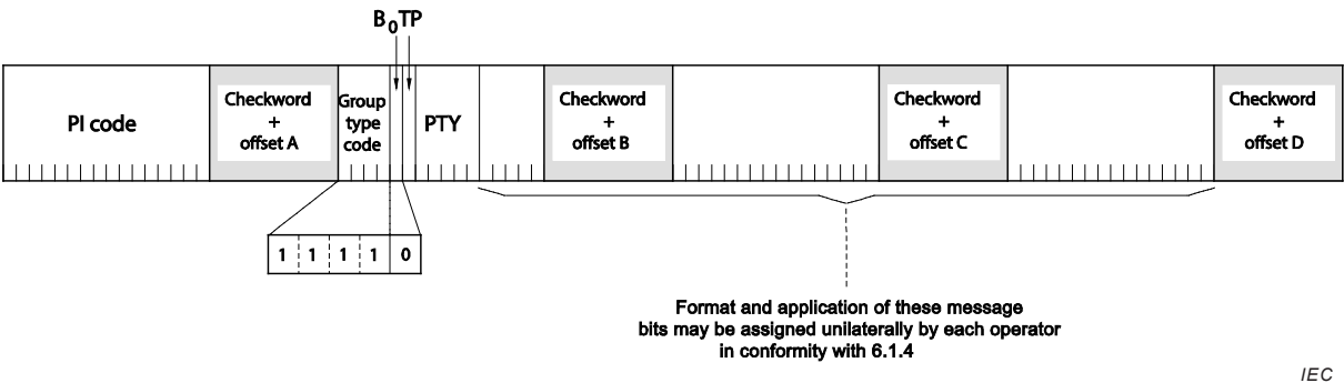
Figure 39 – Open data – Type 15A group
