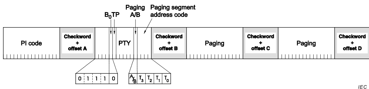
Figure 25 – Radio paging – Type 7A group
