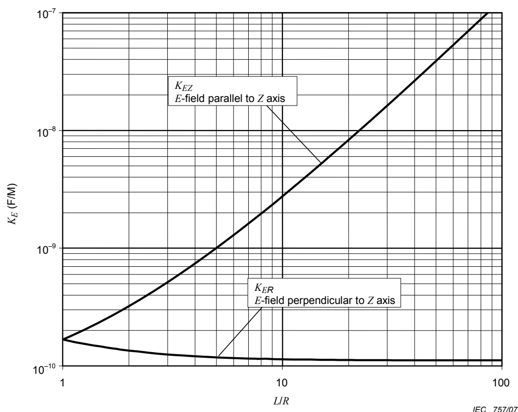
[A1] Figure 8 – Calculation of the shape factor for electric field K_E for a spheroid exposed to an unperturbed electric field [A1]
