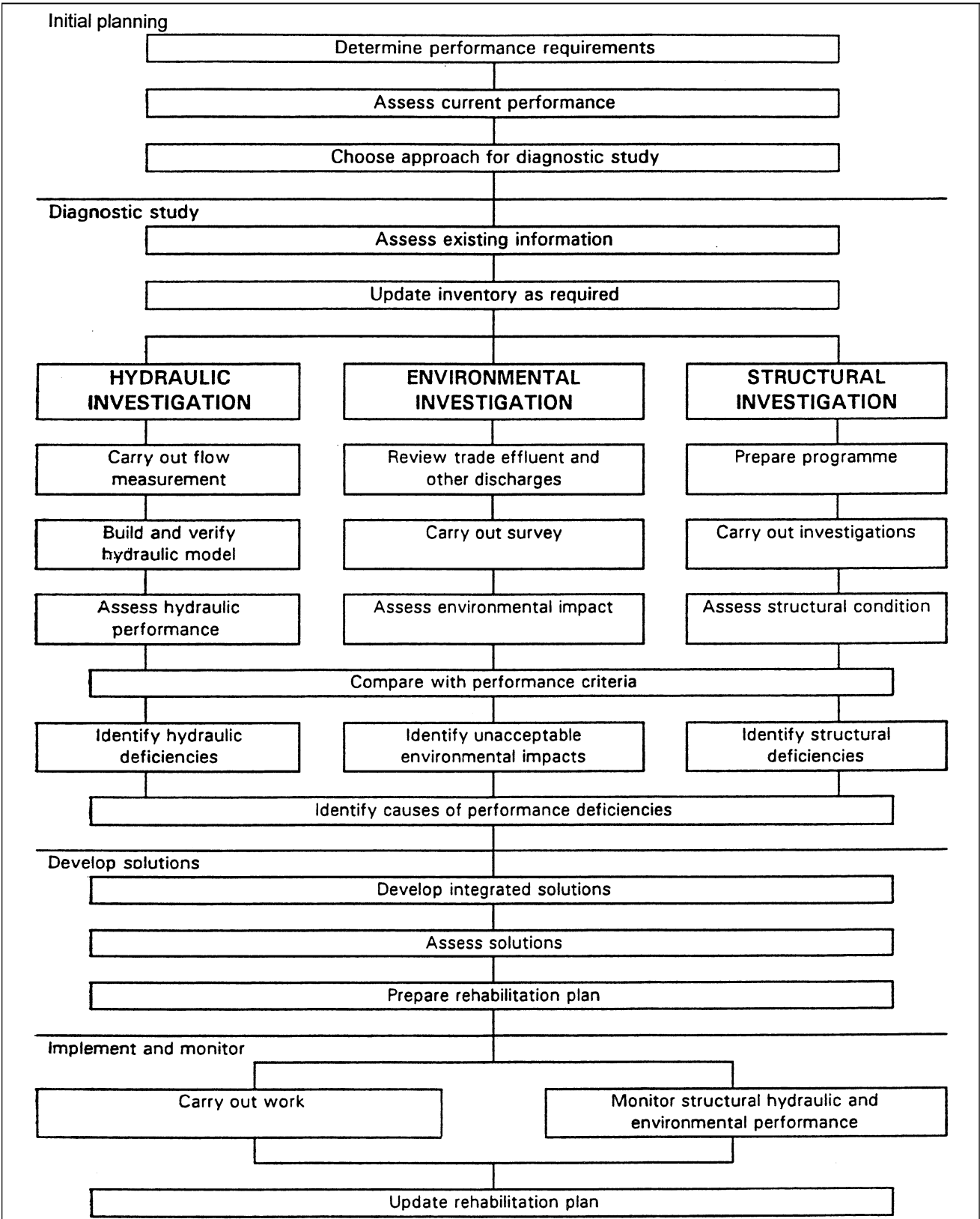
Figure 1. Flow chart for the rehabilitation of drain and sewer systems
