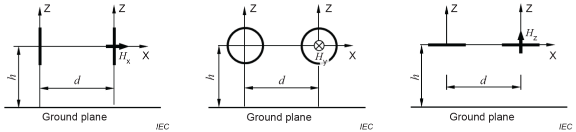
Figure 5 – General arrangement of the three measurement orientations H_x , H_y and H_z , where d is the measurement distance and h is the height of the reference point
