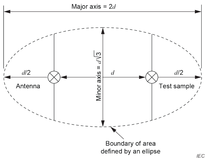
Figure 9 – Obstruction-free area of a test site with a turntable
