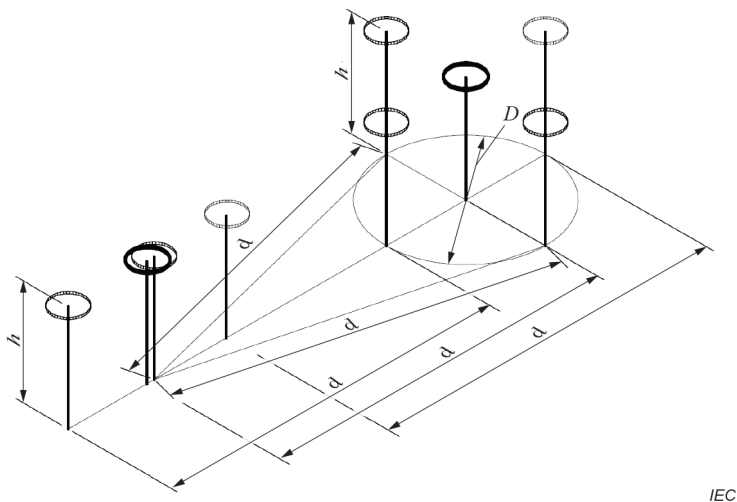
c) H_z validation measurement with loop antennas
