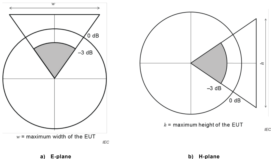
Figure 4 – Determination of maximum useable EUT width using half-power beamwidth
