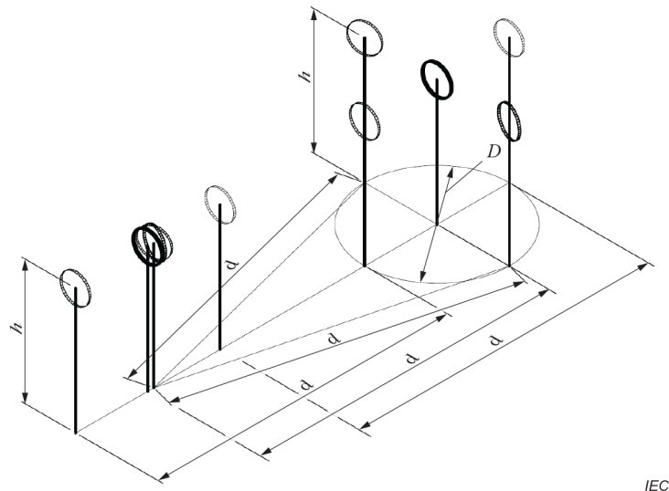
a) H_x validation measurement with loop antennas
