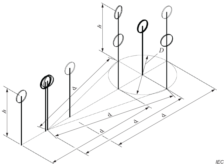
b) H_y validation measurement with loop antennas
