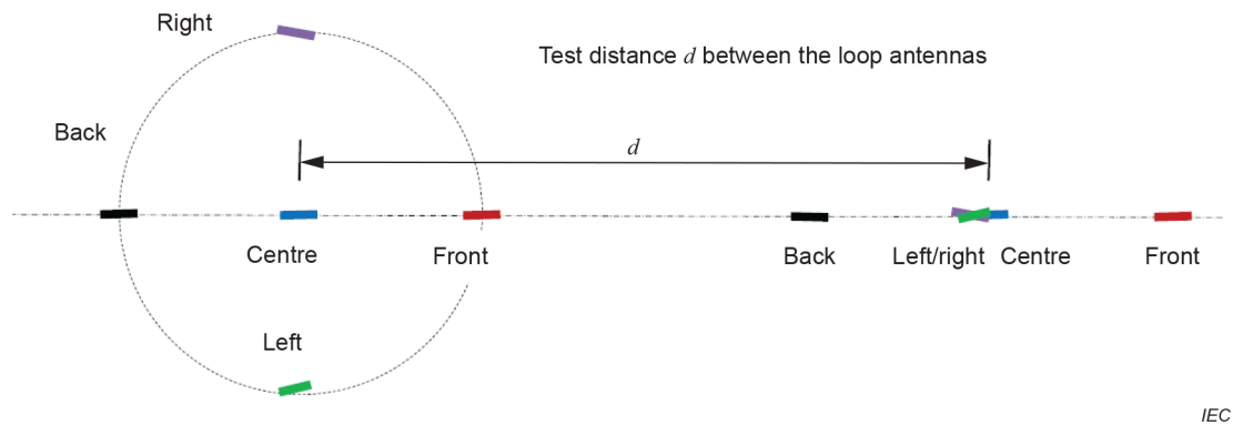
b) H_y validation measurement with loop antennas
