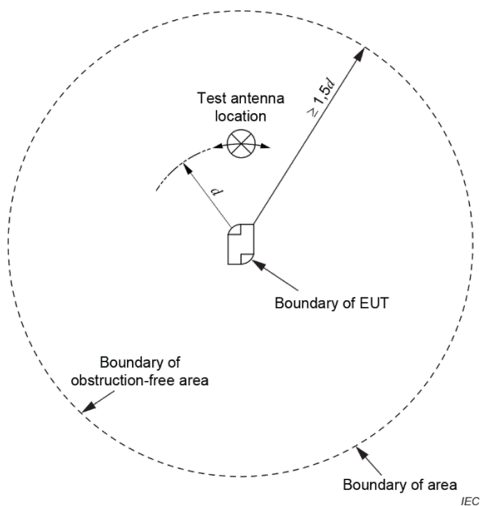
Figure 10 – Obstruction-free area with stationary EUT
