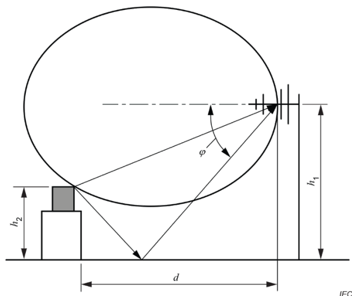
Figure 2 – Schematic of radiation from EUT reaching an LPDA antenna directly and via ground reflection at a 3 m site, showing the beamwidth half-angle, \phi , at the reflected ray
