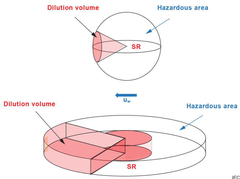
Figure 1 – Dilution Volume
