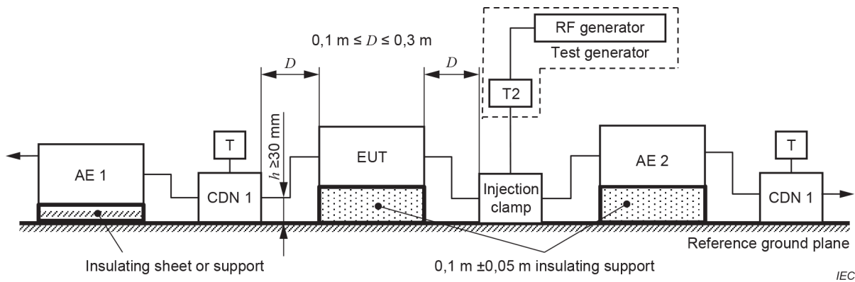
b) Schematic setup for immunity test used for injection clamp
