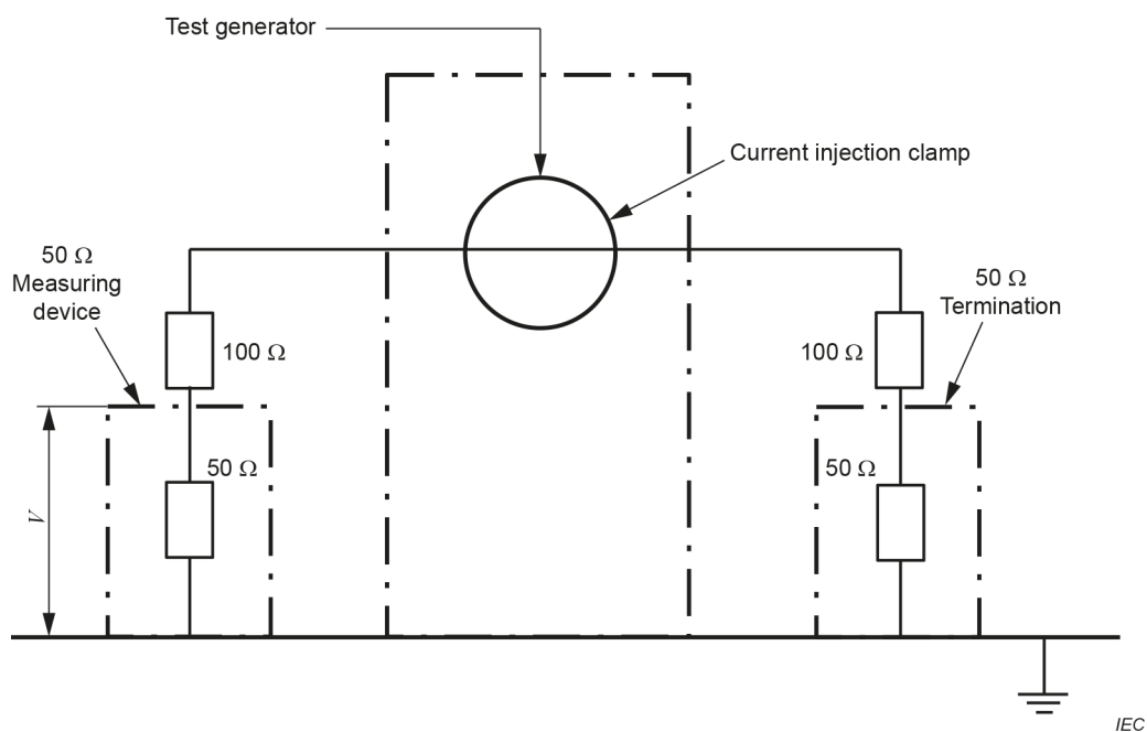
Figure 9 – Example of circuit for level-setting setup in a 150 \Omega test jig
