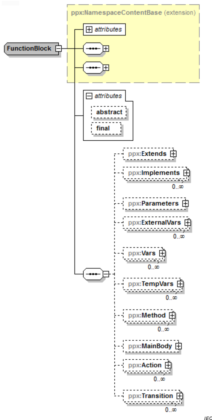
Figure 39 – Complex type "FunctionBlock"
