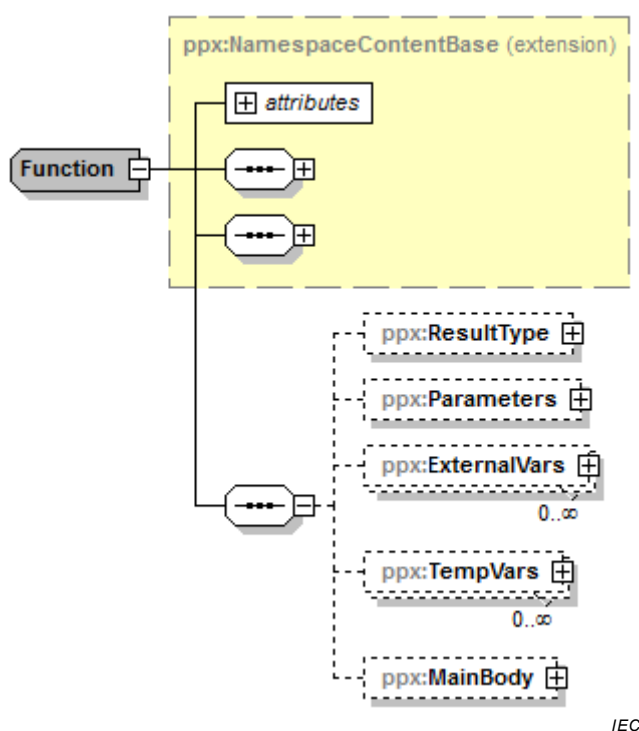
Figure 41 – Complex type "Function"
