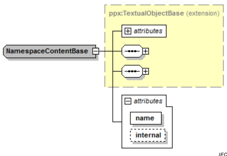
Figure 26 – Complex type "NamespaceContentBase"
