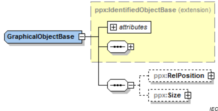
Figure 18 – Complex type "GraphicalObjectBase"
