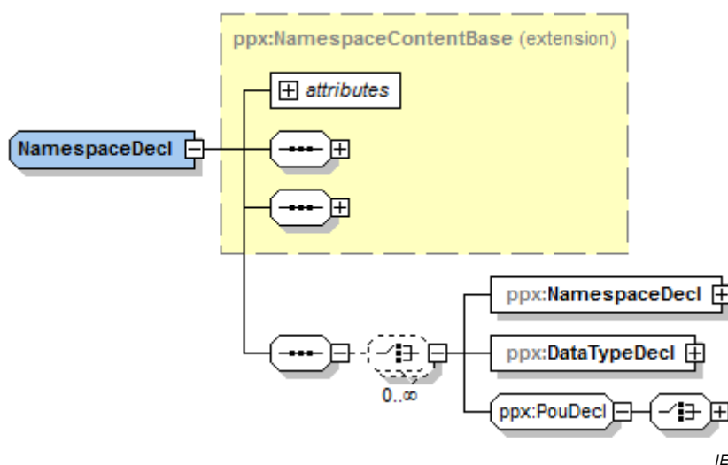
Figure 28 – Complex type "NamespaceDecl"
