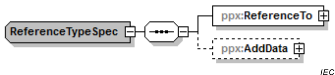
Figure 36 – Complex type "ReferenceTypeSpec"
