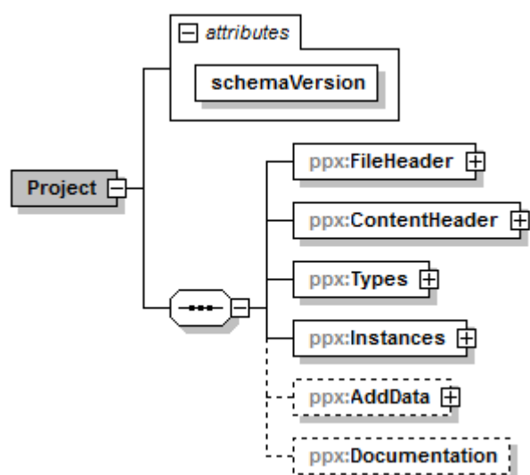
Figure 5 – Main schema element "Project"
