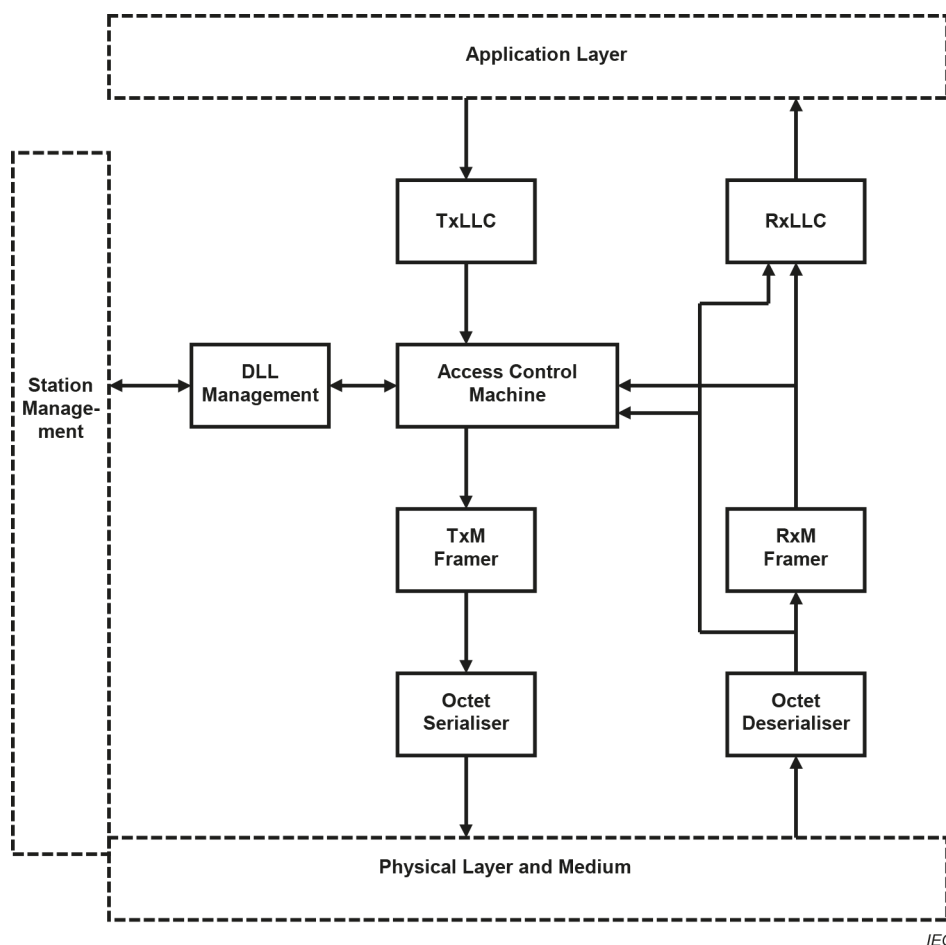
Figure 1 – Data-link layer internal architecture
