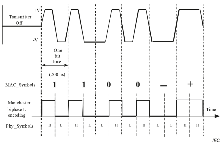
Figure 6 – M_symbols and Manchester encoding at 5 MHz
