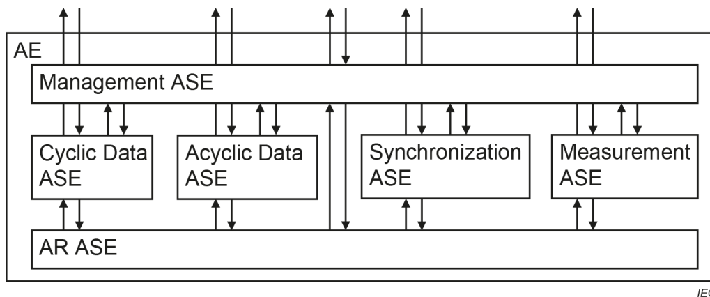
Figure 6 – Structure of ASE type F of FAL Type 23
