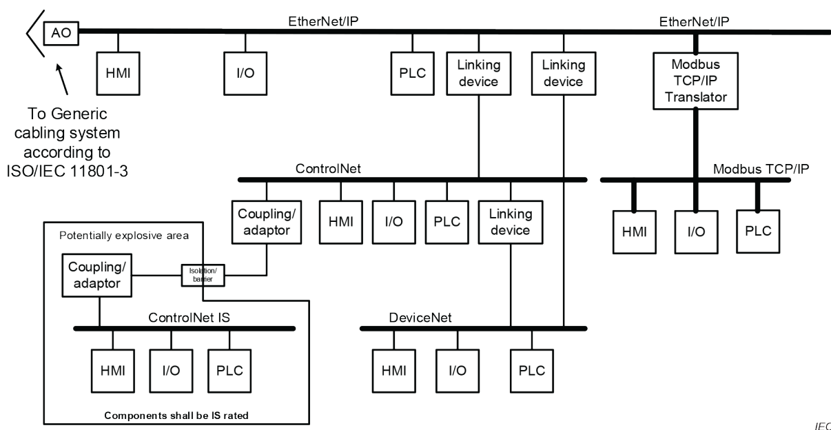
Figure A.1 – Interconnection of CPF 2 networks
