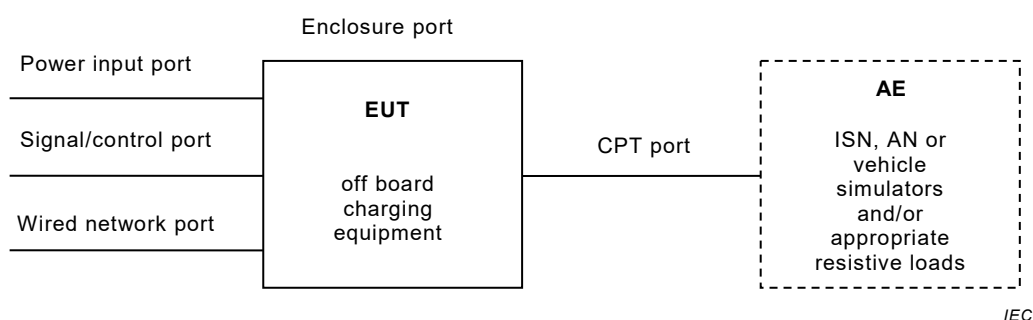
Figure 1 – Examples of ports of off- board charging equipment
