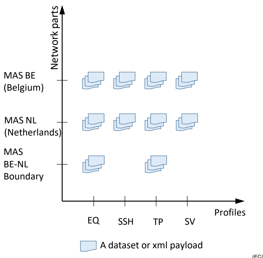
Figure 1 – Relations between MAS, profile and dataset
