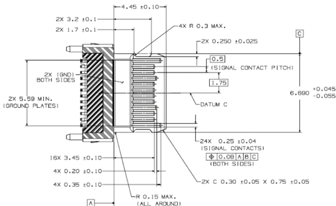
Figure 3-1 USB Type-C Receptacle Interface Dimensions, cont.
