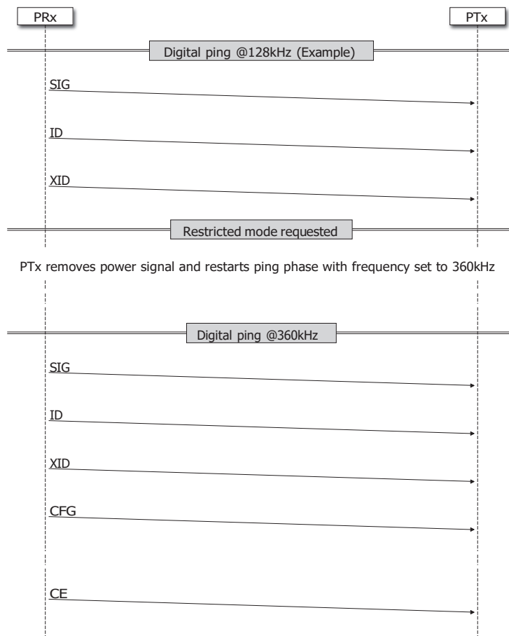
Figure 2.8: MPP Restricted Frequency Change Sequence
