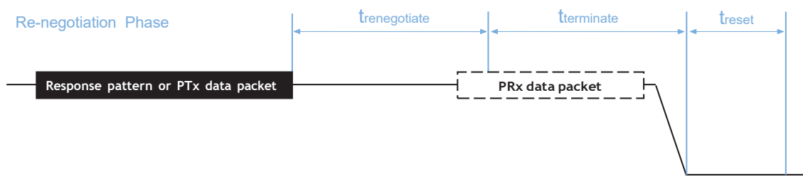
Figure 3.1: Negotiation Phase Timing Parameters - t_{\text{renegotiate}}
