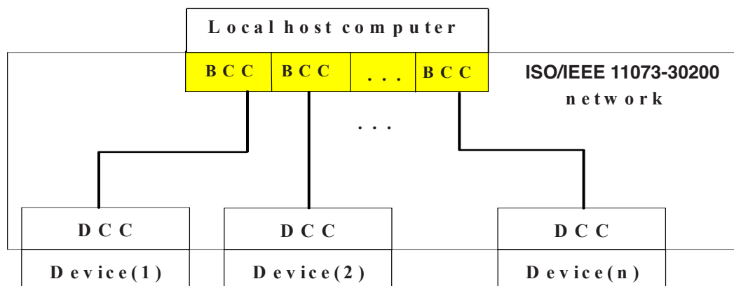
Figure 1 — Connection topology with a local host
