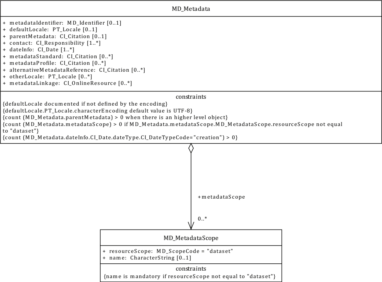
Figure 5 — Metadata on metadata classes
