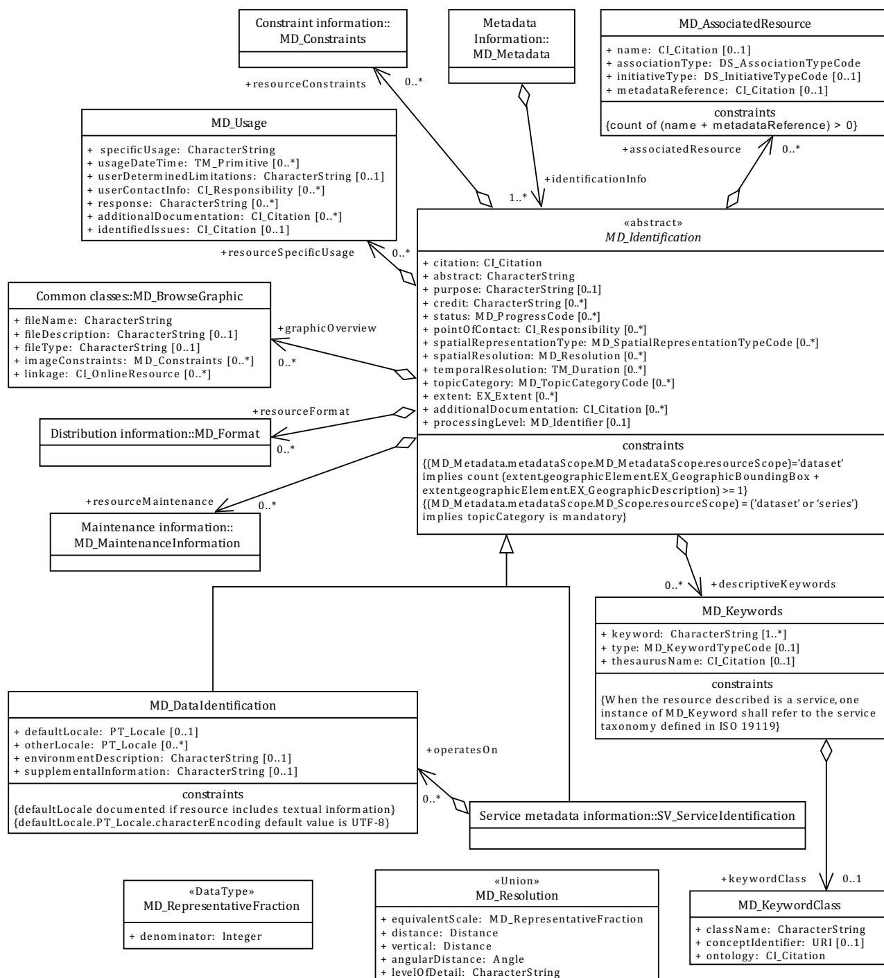
Figure 6 — Identification information classes
