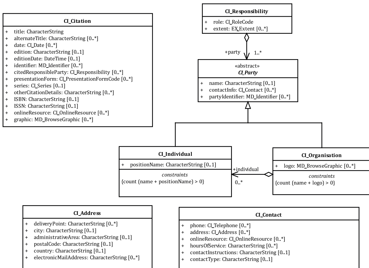
Figure 20 — Citation and responsible party information classes
