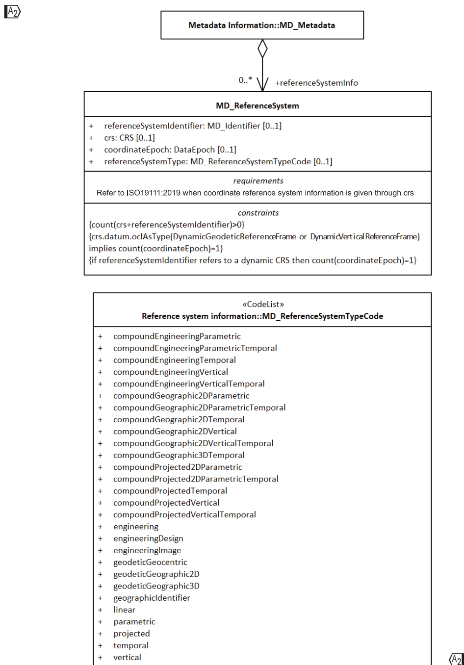
Figure 12 — Reference system information classes
