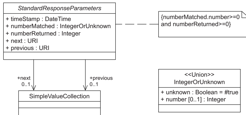
Figure 7 — StandardResponseParameters
