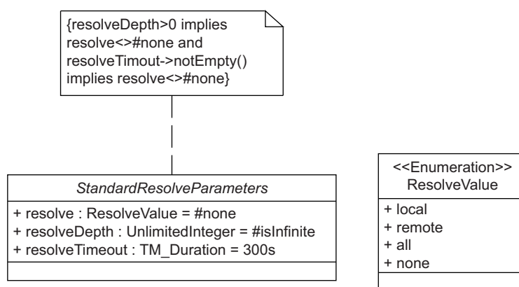
Figure 5 — StandardResolveParameters
