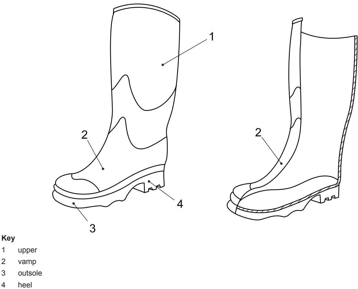
Figure 2 — Example of all-rubber (i.e. vulcanized) or all-polymeric (i.e. entirely moulded) footwear
